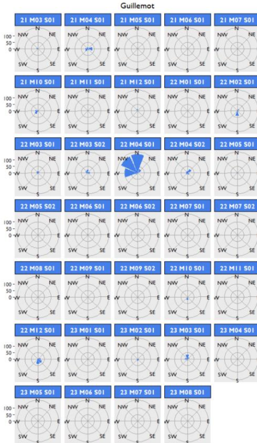
Figure 12.37. Windrose diagrams for months during which flying guillemot were recorded within the array area and a 4km buffer.
